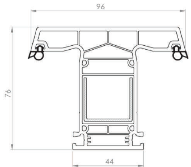
BF 7615 MULLION PROFILE
