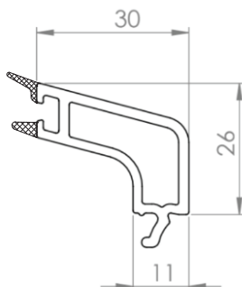
BF 7609 GLAZING BEAD 24 MM
