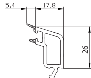
BF 8510 GLAZING BEAD 36 MM
