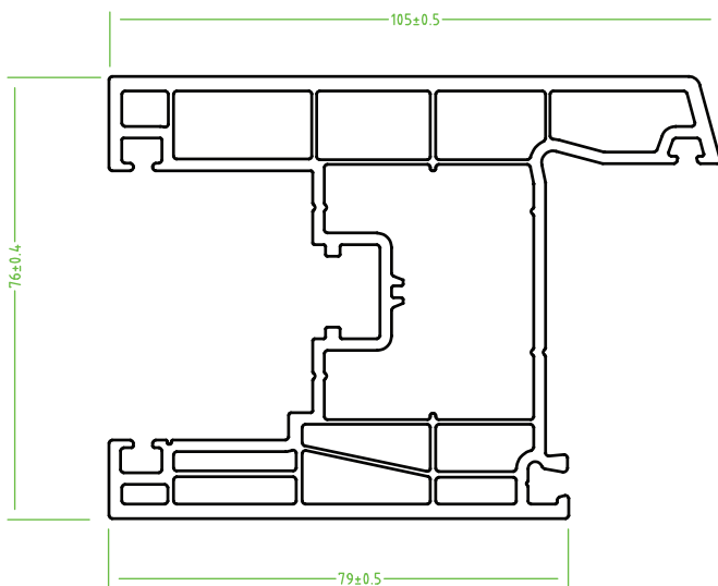
BF 1502 SLIDING SASH
