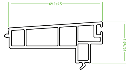
BF 1503 SLIDING FIX FRAME COVER
